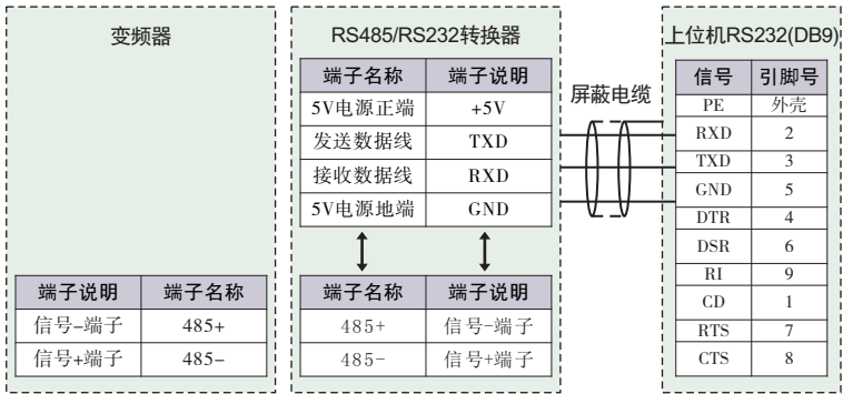
图3-13 RS485-(RS485/232)-RS232通讯配线
