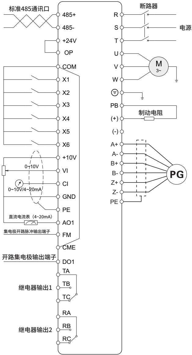
图3-6 基本配线图 (V9-4T0110G ~ V9-4T0220G)
