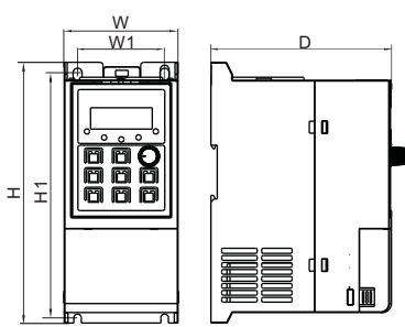
2S0007G~3.7G / 4T0007G~2.2G外观尺寸图
